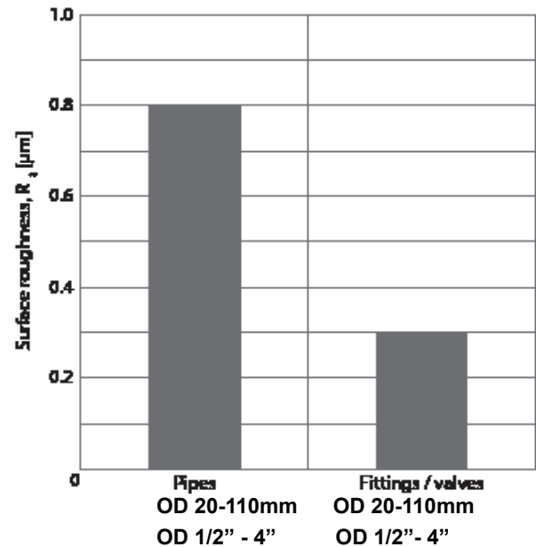
Figure D-16. Surface specification for PolyPure® pipes
