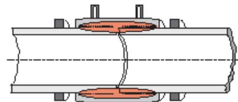
Figure E-25. Completed electrofusion weld
