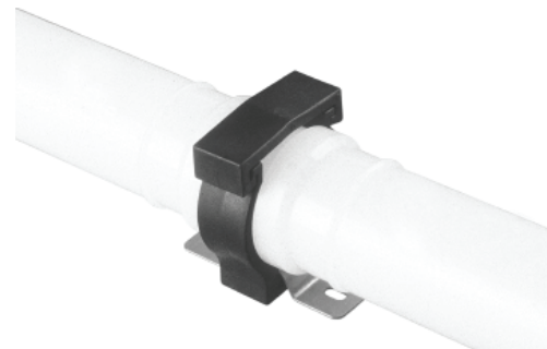
Figure D-25. Anchor and restraint fitting support
