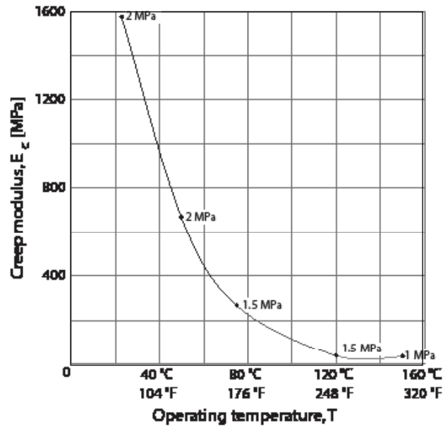
Figure D-11. Creep modulus curves for E-CTFE
