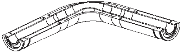
Figure F-10. Impeded heat expansion design
