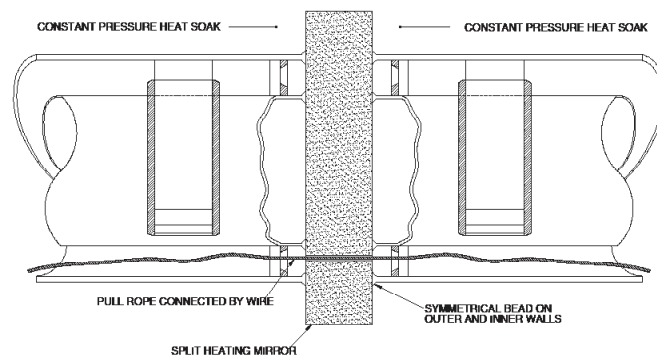
Figure E-17. Pipe ends heated with pull rope installed
