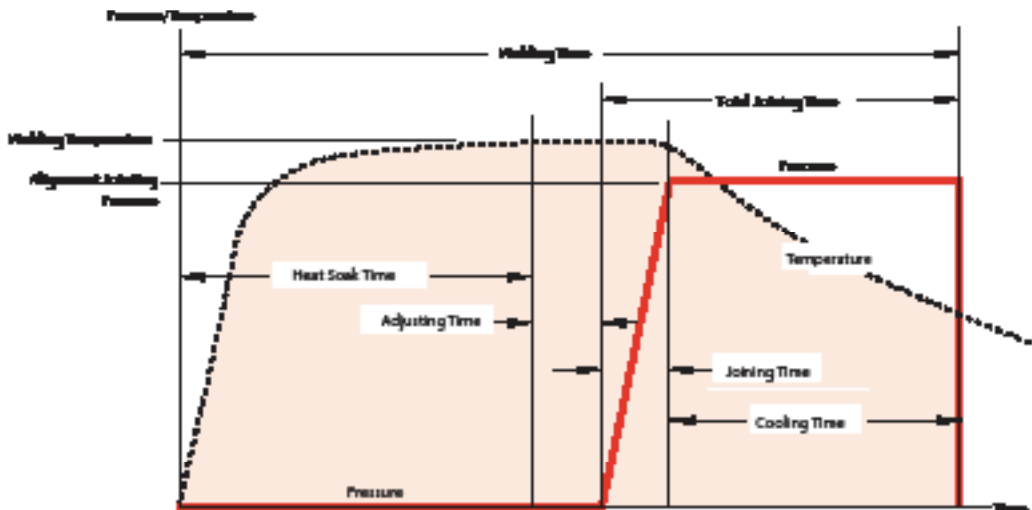
Figure E-21. IR fusion timing diagram
