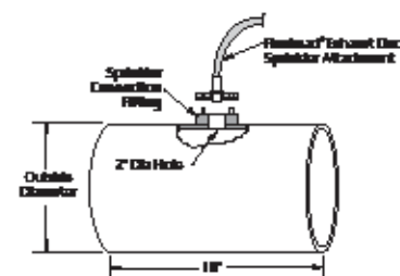
Figure F-11. Detail of a flexible sprinkler head and mounting component
