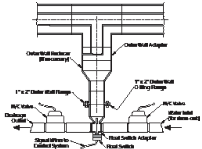
Figure G-18. Drain and low-point Poly-Flo® system
