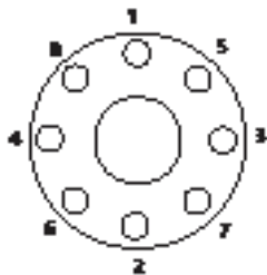
Figure E-33. Torque pattern
