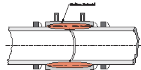
Figure E-24. Molten material from both coupling and pipes form weld
