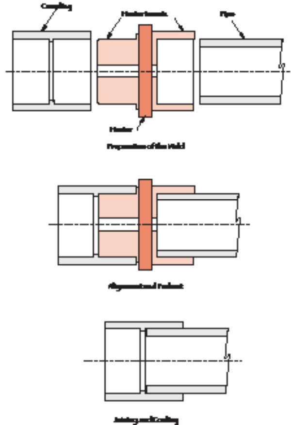
Figure E-2. Socket Fusion Welding Process
