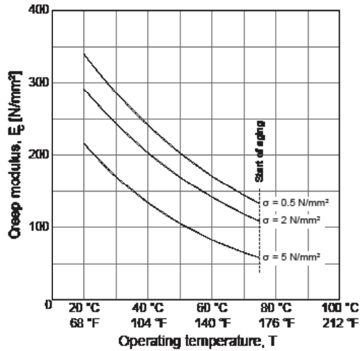
Figure D-1. Creep modulus curve for PE100 at 1 year
