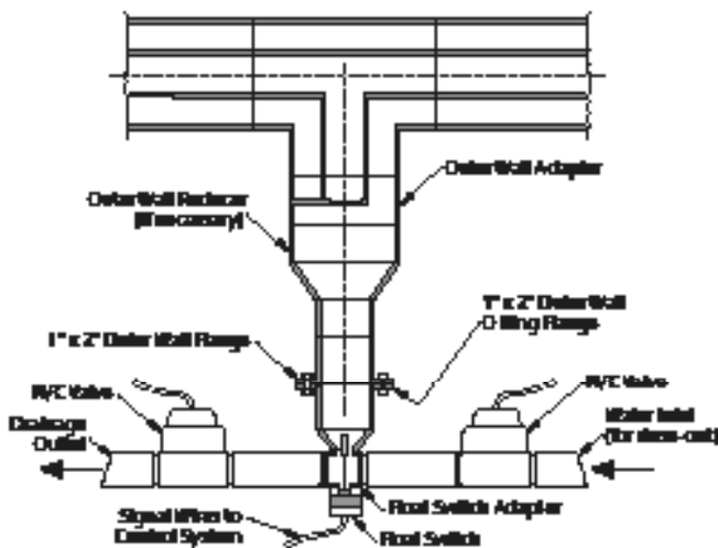
Figure G-13. Drainage of containment pipe: Poly-Flo® system with low point sensor
