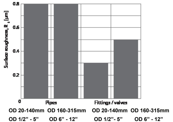
Figure D-15. Surface specification for PP-Pure® pipes
