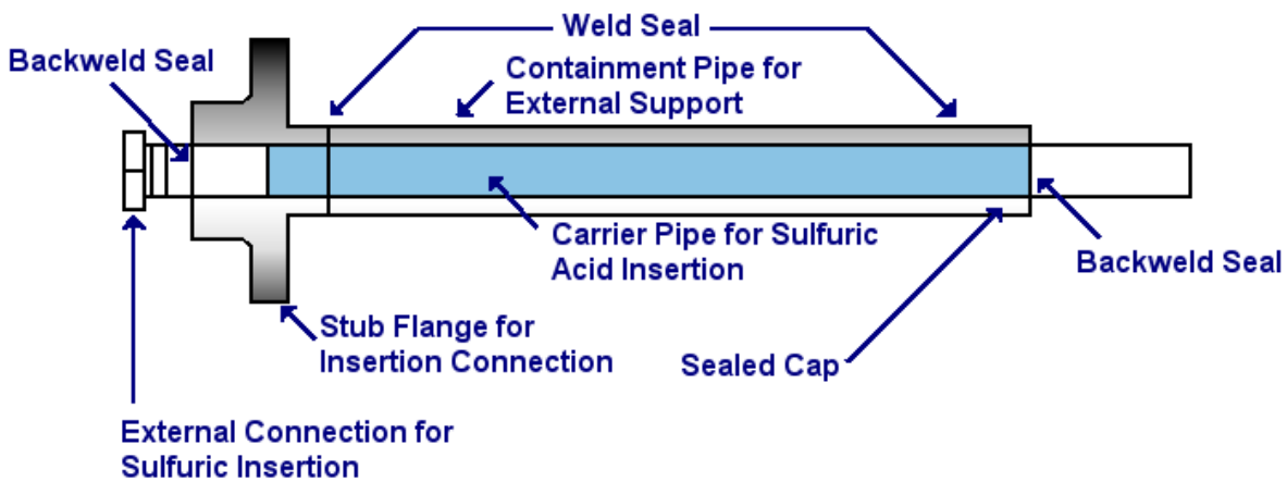
Figure 2: Injection quill, which will inject the chemical into the center of the pipe, creating a better blend of acid in the water.
